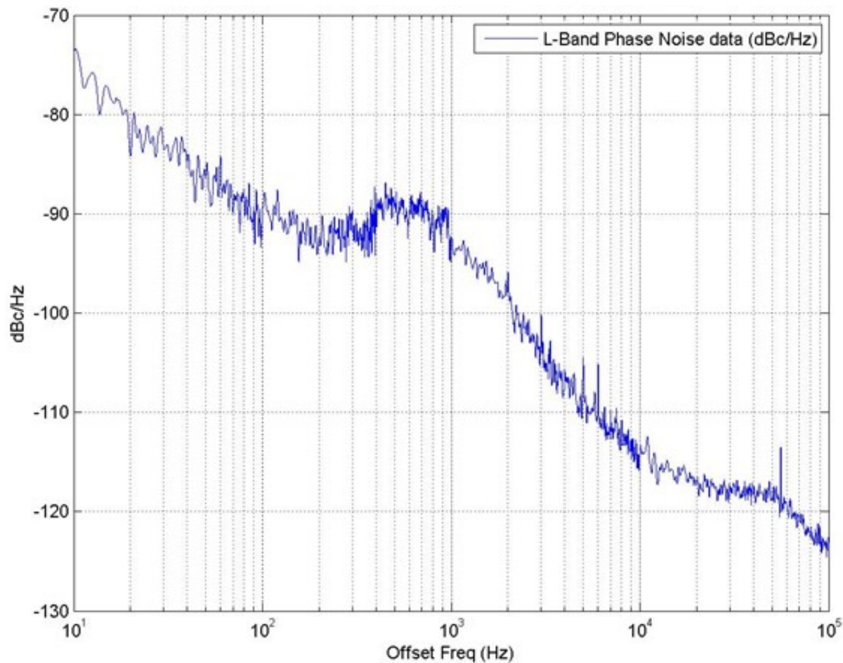
Figure 6-2 Typical GPS III L5 Carrier Phase Noise Spectral Density
