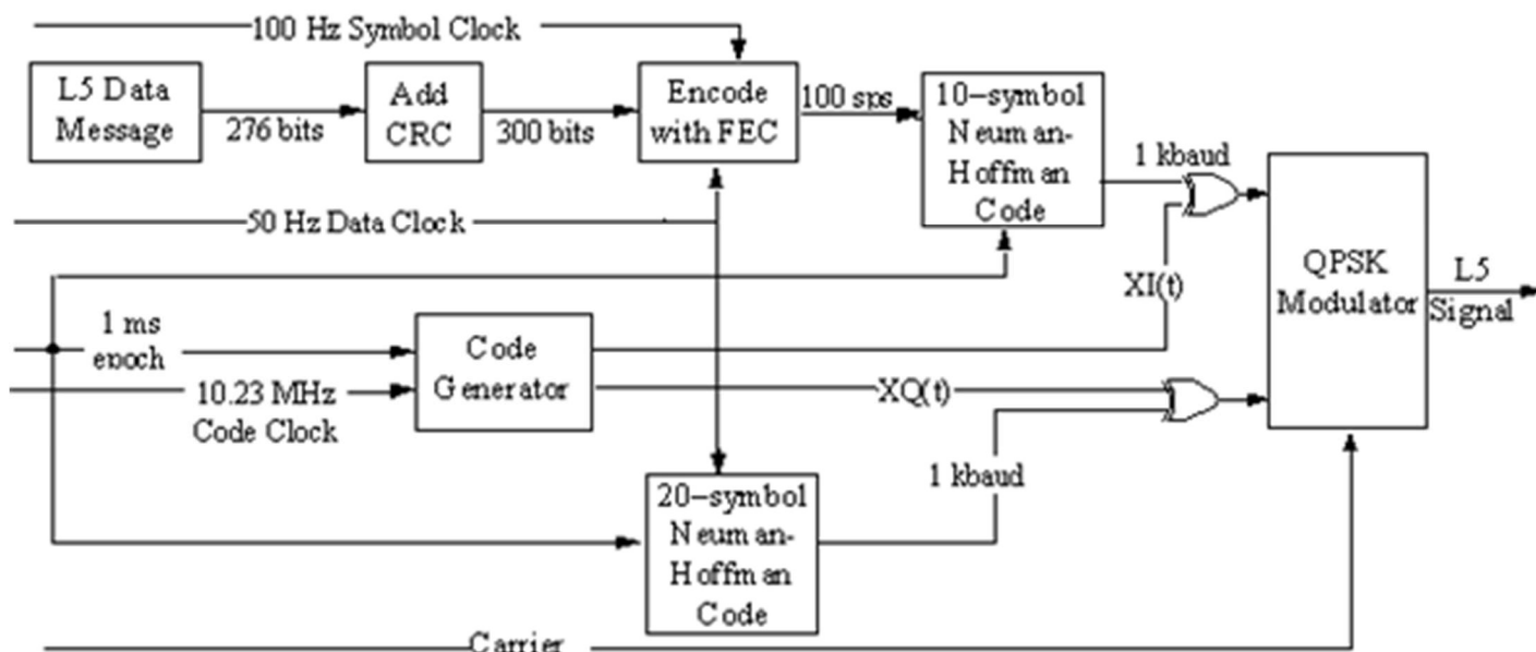
Figure 3-3. Modulation of Signals
